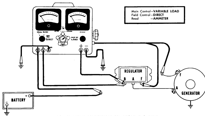
DIAGRAM SHOWS CONNECTIONS FOR NEGATIVE GROUND REVERSE VOLTMETER LEADS FOR POSITIVE GROUND
